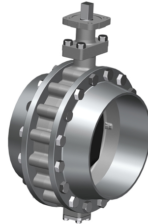
3D drawing of DANAIS 150 T4 (with extension option)
